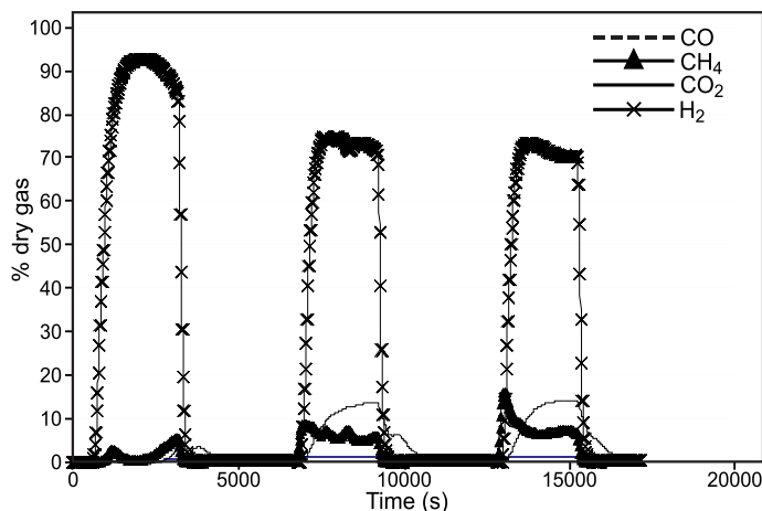
Figure 9: Dry reformat gas composition for three initial cycles sunflower oil+steam feed/air feed in conditions of Figure 8ab. In order of decreasing content: H_2 > CO_2 > CH_4 > CO .
