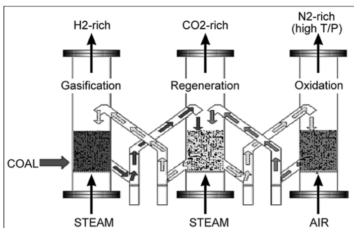
Figure 3: Schematic of operation of the UFP (from Rizeq et al. , 2003)
