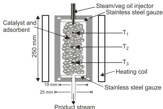
Figure 5: Close up diagram of USR reformer reactor at Leeds University
