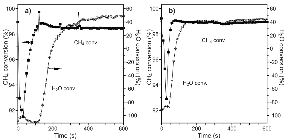
Figures 6a-b: Methane and steam percent conversions during FF (fuel/steam flow step) on 40 g of OTM 'A' (Ni content of 27.5 wt% on alumina) for a reactor temperature of 800°C, at a steam/methane molar ratio of 1.8 using a step duration of 600 s (a) methane flow of 152 sccm ( 1.13 \times 10^{-4} mol of C/s) and (b) 400 sccm ( 3 \times 10^{-4} mol of C/s). These runs were without CO_2 sorbent. (Dupont et al., 2006)
