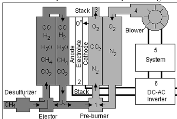
Figure 11: Diagram of operation of a Solid Oxide Fuel Cell fuelled by natural gas. A reformate fuelled SOFC would not need the pre-reformer on the left hand side. (Ben Wiens Energy Science Inc., 2006)
