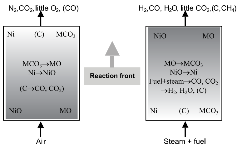
Figure 2: Sequence of the main reactions under the two feed steps.
