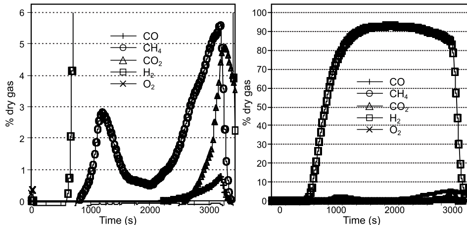
Figures 8a-b: Dry reformate composition for conditions of Table 6 (steam/sunflower oil feed, ratio of 4) this time with dolomite mixed with Ni-OTM 'A' present in the USR reformer reactor. Figure 8a: lower scale emphasises the minor reformate products (CO, CO 2 , CH 4 , O 2 ), Figure 8b: larger scale shows the major reformate product hydrogen
