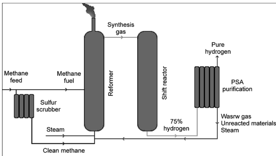
Figure 1: Methane steam reforming illustration. PSA= pressure swing adsorber (removes \text{CO}_2 from the reformat and produces a pure \text{H}_2 stream).
