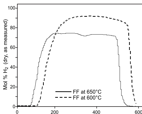
Figure 7: \text{H}_2 content in reformate (on a dry basis) when using a reactor set temperature of 600°C (dashed line) and 650°C (solid line) during FF step, over 64 g of OTM 'A' and 21 g of dolomite homogeneously mixed. The flow of methane was maintained at 200 sccm, with a steam to carbon ratio of 4.
