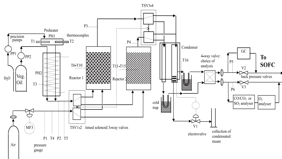
Figure 10: Diagram of pilot scale USR for continuous production of H 2 used to feed a SOFC
