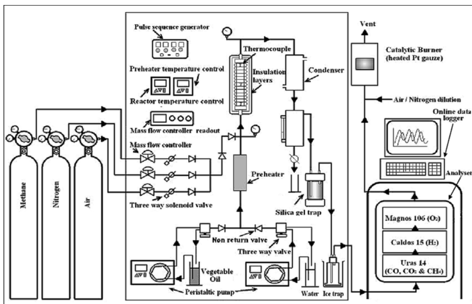
Figure 4: Diagram of bench scale USR set up at Leeds University
